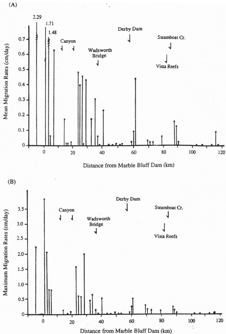
Figure 4. Downstream variations in (A) mean channel migration rates, and (B) maximum channel migration rates. Mean rates are calculated as the average of three measurements made at 100 m intervals at each site, whereas maximum rates represent the largest values observed at each location.
