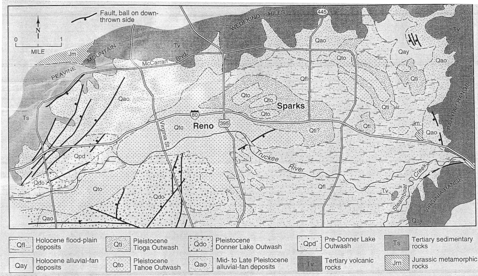
Generalized surface geology of the northern Truckee Meadows (modified after Bell and others, 1984).
